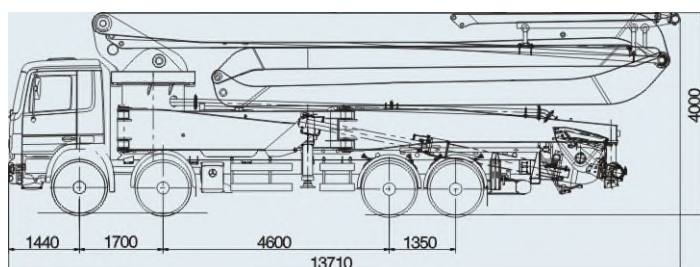
Dimensions varying according to truck assembly
