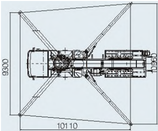
Full Support
