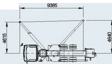
Lateral Support
