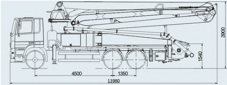
Dimensions varying according to truck assembly
